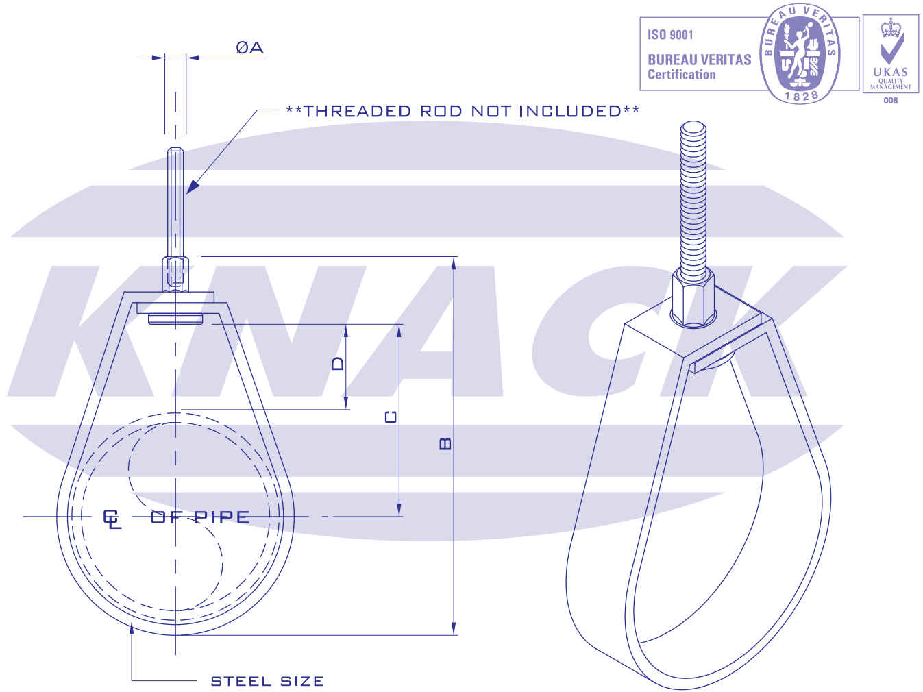
FIGURE H 521 ADJUSTABLE SWIVEL RING
