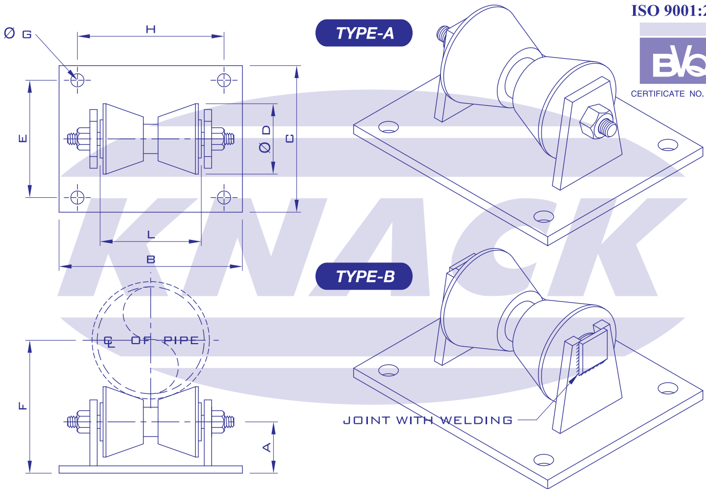
FIGURE H 562 STEEL ROLLER STAND
