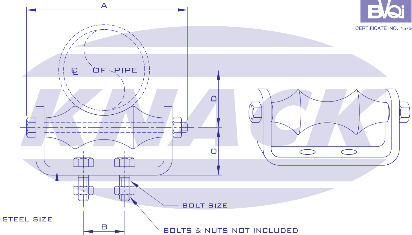
FIGURE H 561 ROLLER CHAIR
