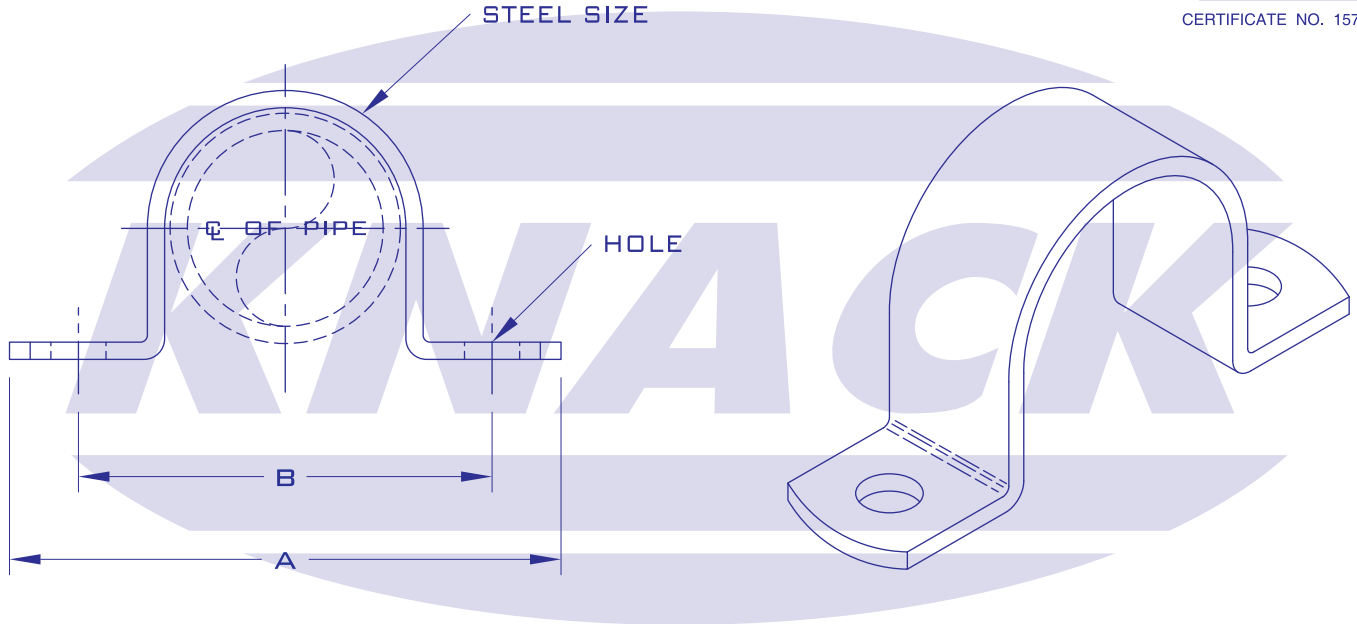
FIGURE H 551 STANDARD SHORT PIPE STRAP
