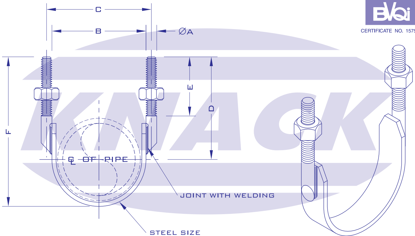
FIGURE H 542 STRAP U-BOLT
