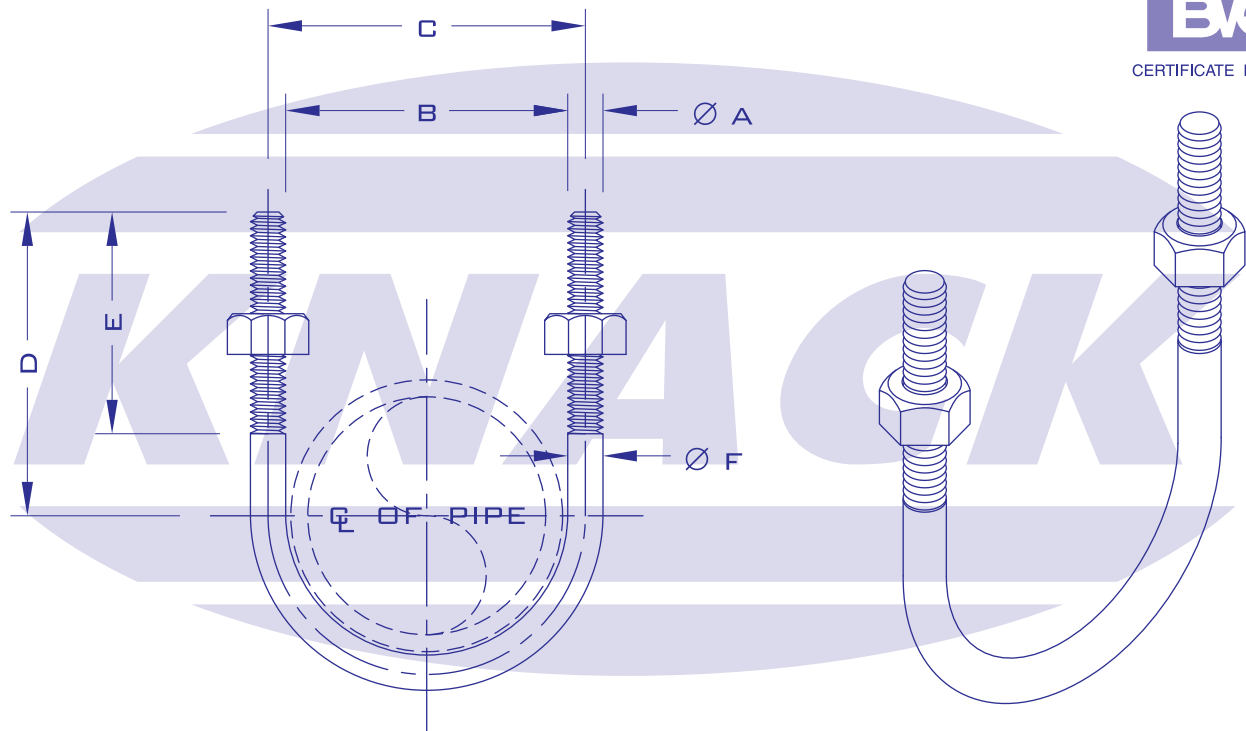
FIGURE H 541 STANDARD U-BOLT
