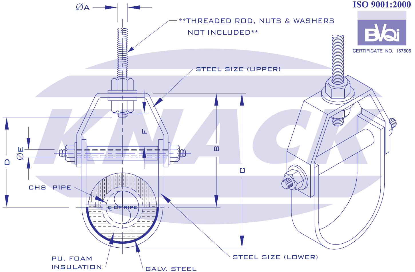
FIGURE H 531-N ADJUSTABLE CLEVIS HANGER (P.U.FOAM INSULATION)
