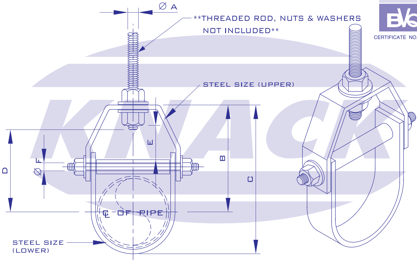
FIGURE H 531 STANDARD ADJUSTABLE CLEVIS HANGER
