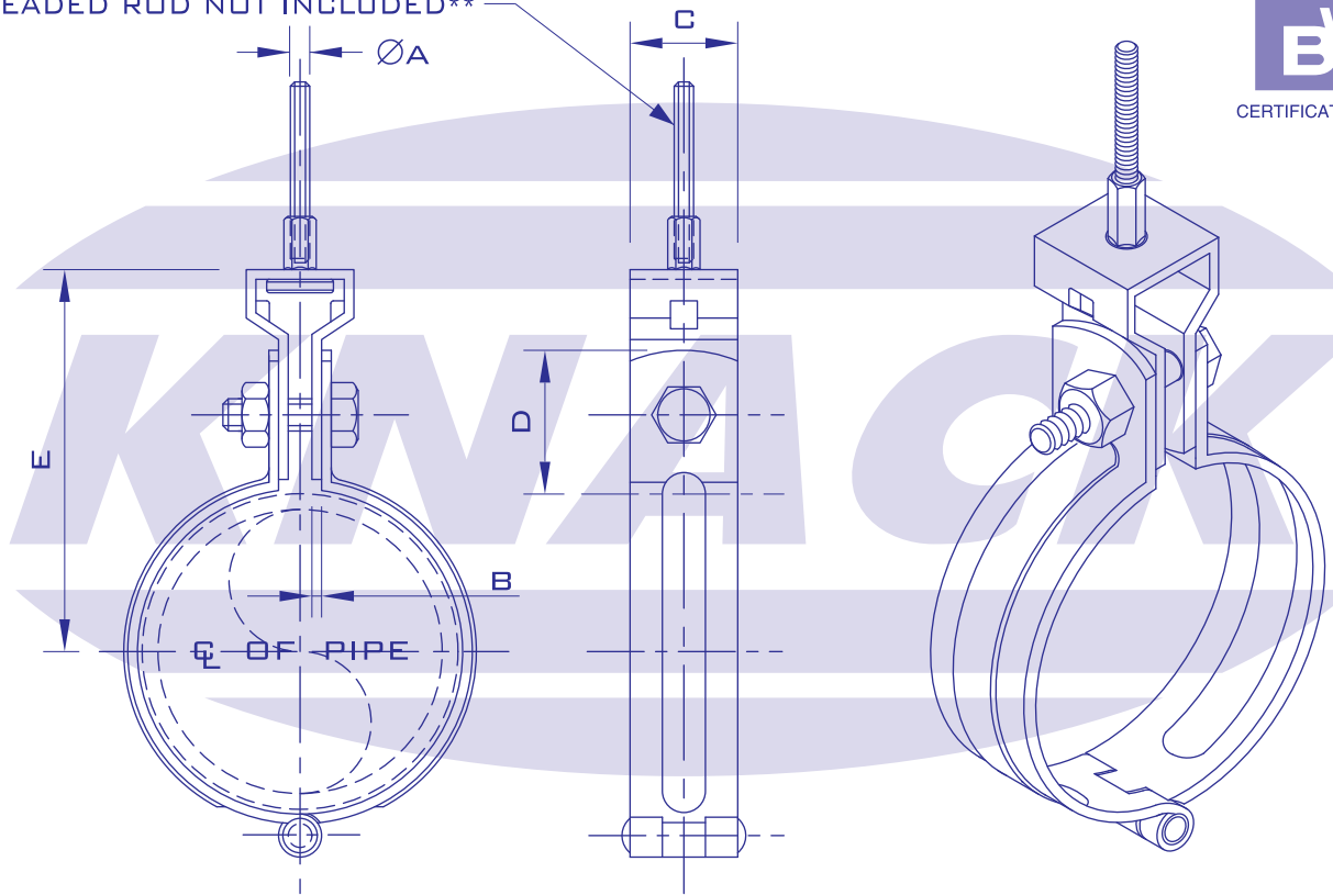
FIGURE H 523 SPLIT RING HANGER WITH SWIVEL ADJUSTABLE
