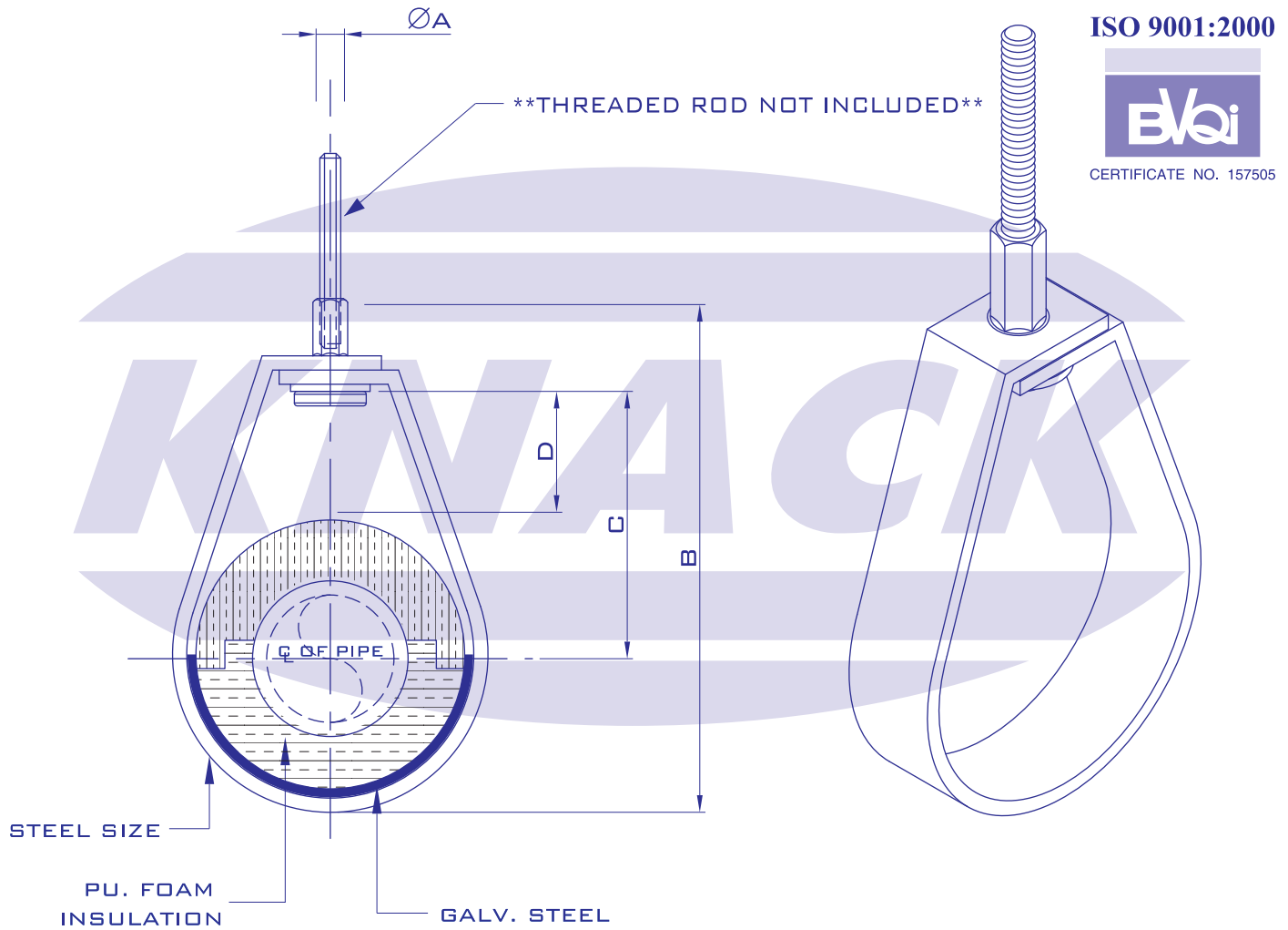
FIGURE H 521-N ADJUSTABLE SWIVEL RING (P.U.FOAM INSULATION)
