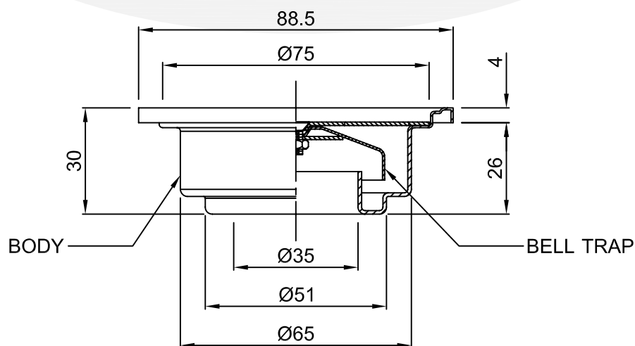
SECTION A - B
