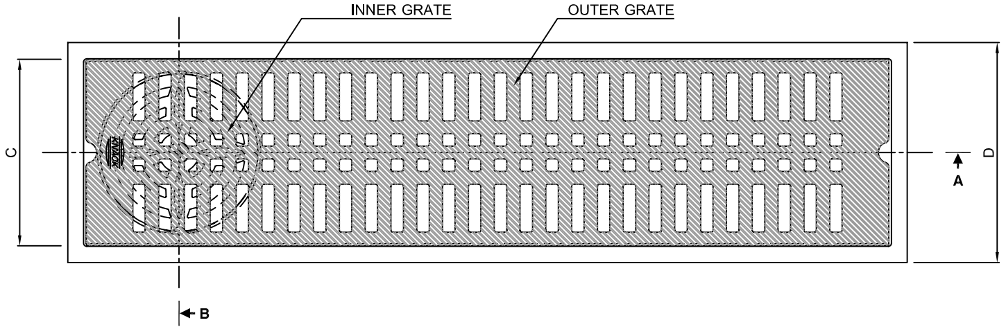
TOP VIEW
