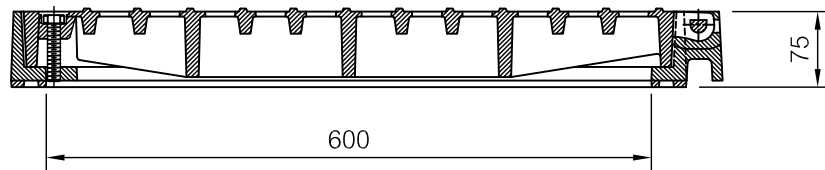
SECTION B-B
