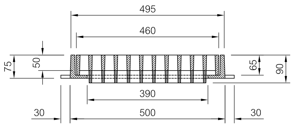
SECTION A - A SCALE 1 : 7.5
