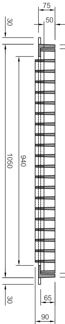
SECTION A - A SCALE 1 : 10
