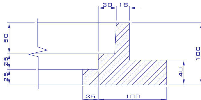
DETAIL "B"
